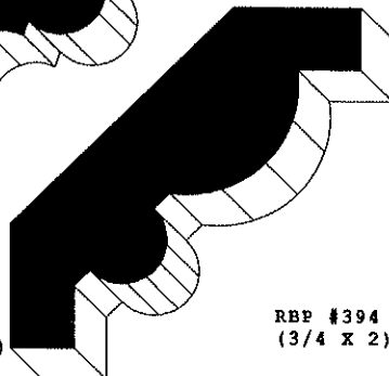
RBP #316 (3/4 X 2-3/4)
