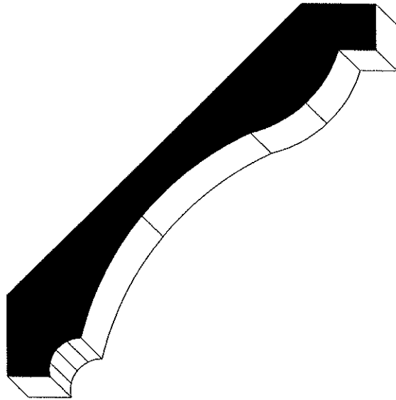
RBP #391 (3/4 X 4-1/2)
