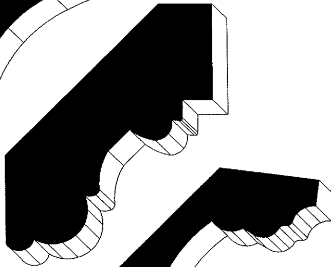
RBP #3068 (1-1/4 X 3-3/4)
