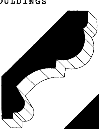
RBP #3070 (3/4 X 2-3/4)
