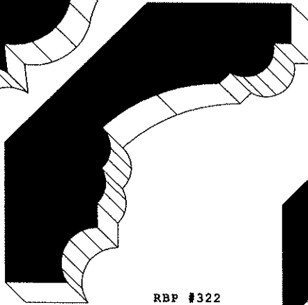
RBP #322 (3/4 X 3-1/8)
