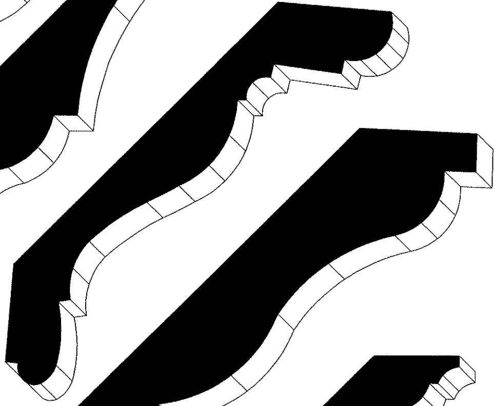
RBP #3090 (1-3/16 X 5-7/8)
