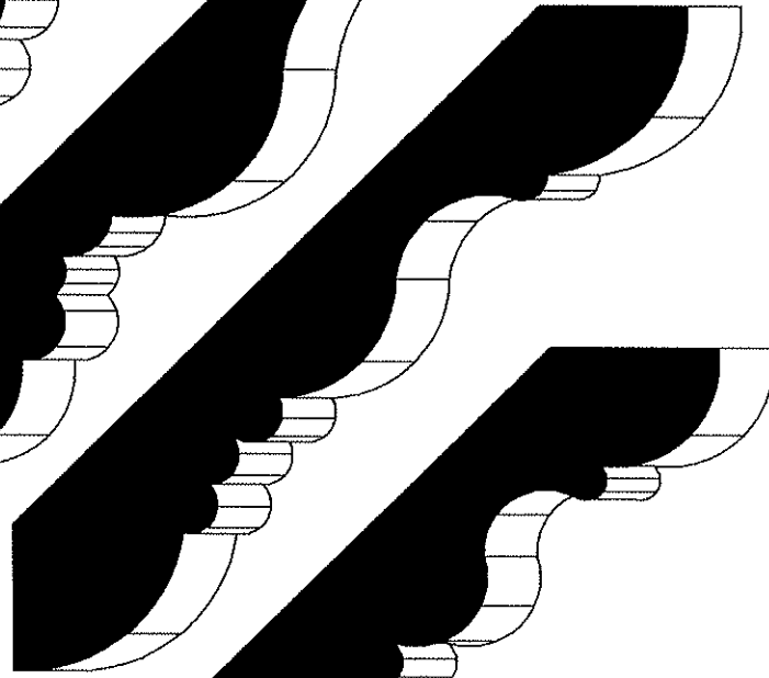
RBP #348 (3/4 X 4-1/2)
